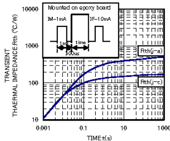
Rth-t CHARACTERISTICS
