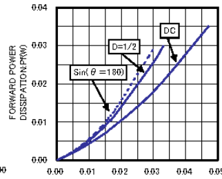
AVERAGE RECTIFIED FORWARD CURRENT I_o -PF CHARACTERISTICS
