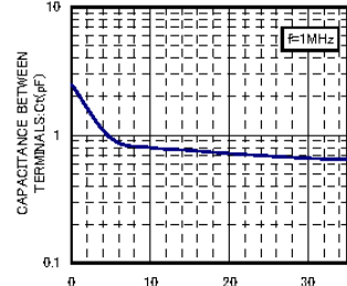
VR-Ct CHARACTERISTICS
