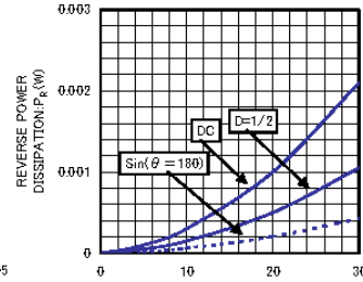
REVERSE VOLTAGE V_R - P_k CHARACTERISTICS
